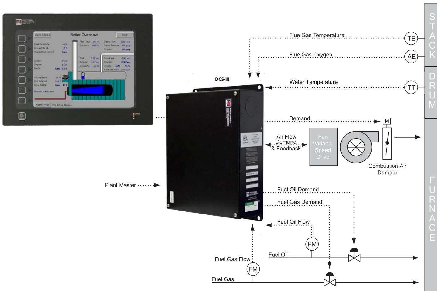
Model BMTS-HWFMC Combustion Control System
