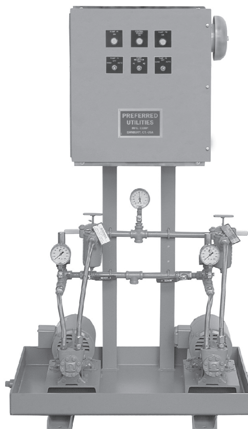
Semi-Automatic Fuel Oil Transfer Pump Set
